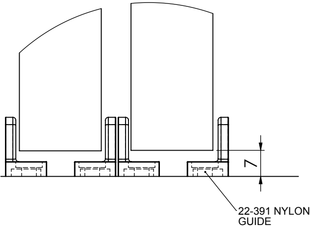
GUIDES SURFACE FIXED
